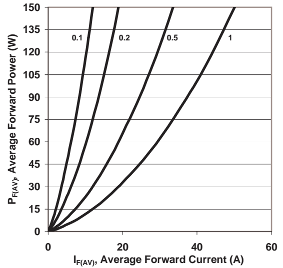
Figure 4. Typ. Forward Power Dissipation vs. Average Forward Current
