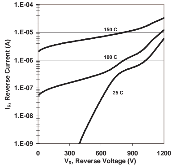
Figure 2. Typ. Reverse Characteristics I_R = f(V_R)
