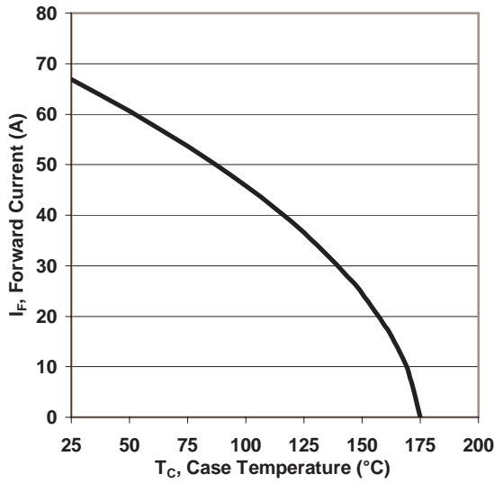
Figure 3. Diode Forward Current I_F = f(T_C); T_j < 175\text{ }^\circ\text{C}; R_{th,JC(max)}
