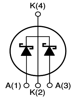
Internal Schematic
