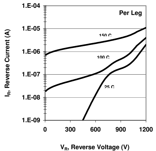
Figure 2. Typ. Reverse Characteristics I_R = f(V_R)
