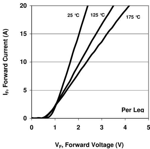
Figure 1. Typ. Forward Characteristics I_F = f(V_F) ; parameter: T_j
